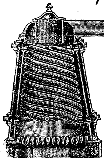
Section of New Patent Combined Conical Tubular Boiler.
